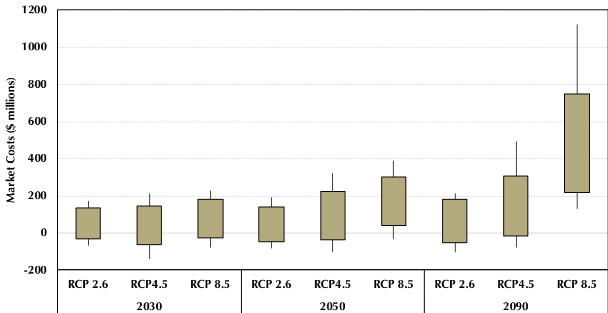
FIGURE 11 "Market" Costs Associated with Changes in Mortality in Maryland in the 21st Century
