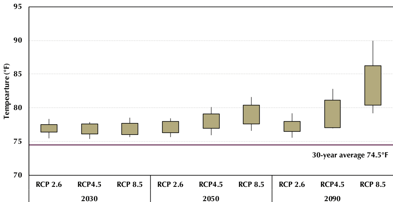
FIGURE 2: Projected Changes in Average Summer Temperature in Maryland in the 21st Century
