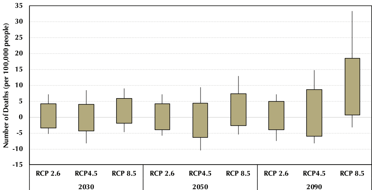
FIGURE 9: Projected Changes in Mortality in Maryland in the 21st Century
