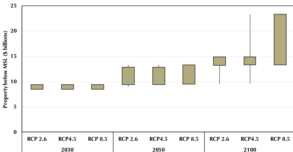
FIGURE 12: Increases in Coastal Property at Risk of Inundation in Maryland for 2030, 2050, and 2100
