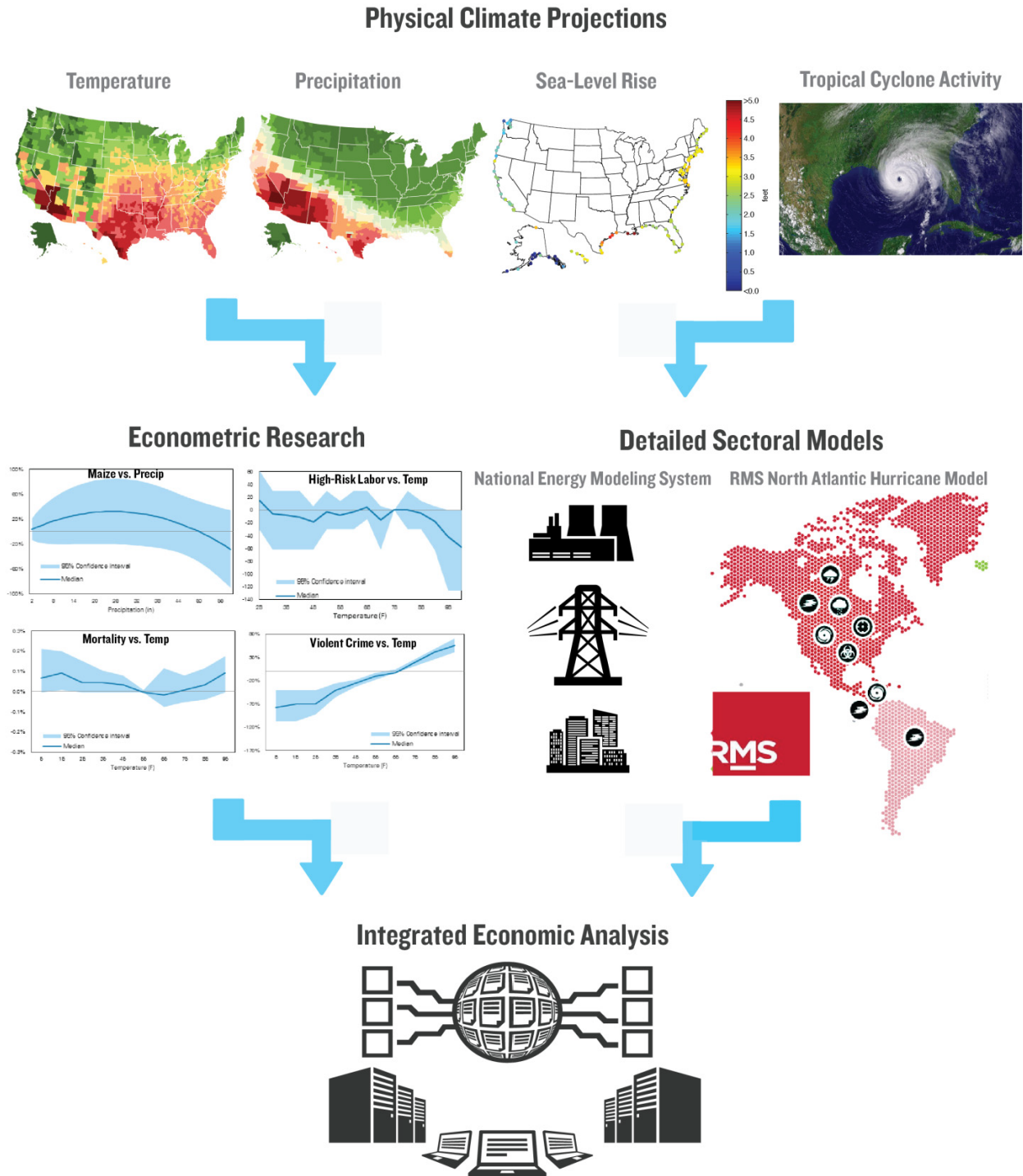
FIGURE 1: A Schematic Depicting the Methodology Used in the American Climate Prospectus
