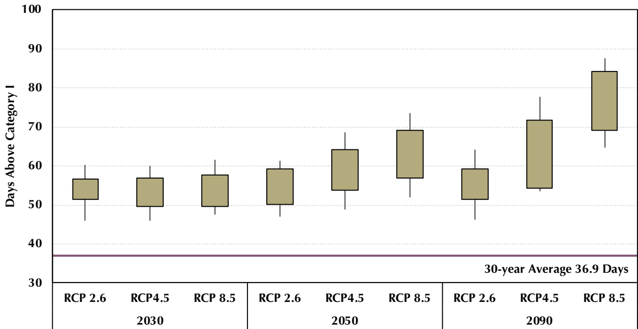
FIGURE 6: Projected Changes in the Number of HHSI I Days in Maryland in the 21st Century
