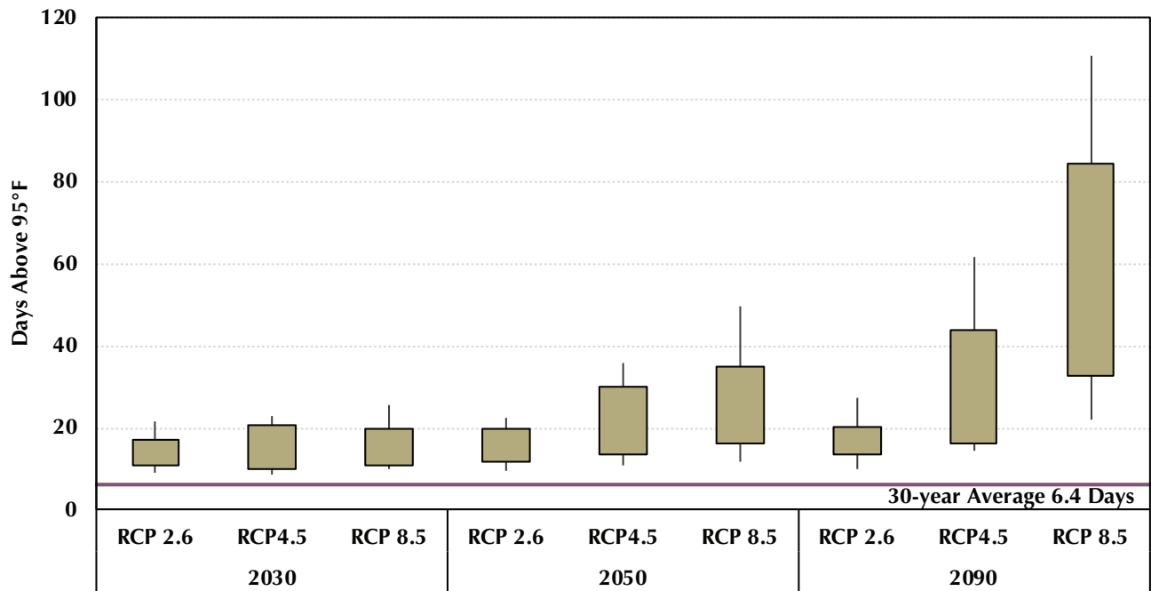
FIGURE 4: Projected Changes in Number of Days above 95°F in Maryland in the 21st Century
