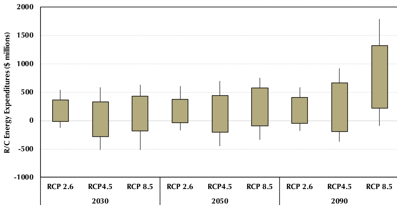
FIGURE 17: Changes in Energy Expenditures in Maryland in the 21st Century
