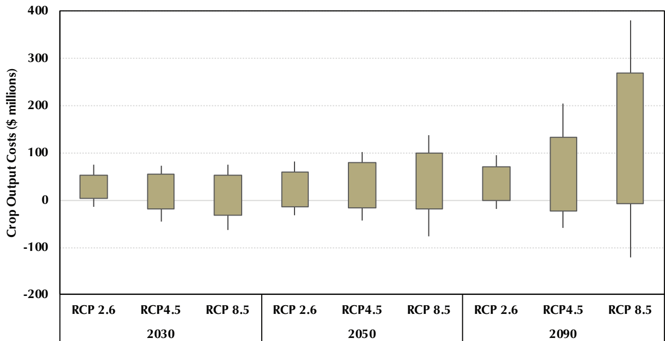
FIGURE 19: Costs Associated with Changes in Crop Yields in Maryland in the 21st Century
