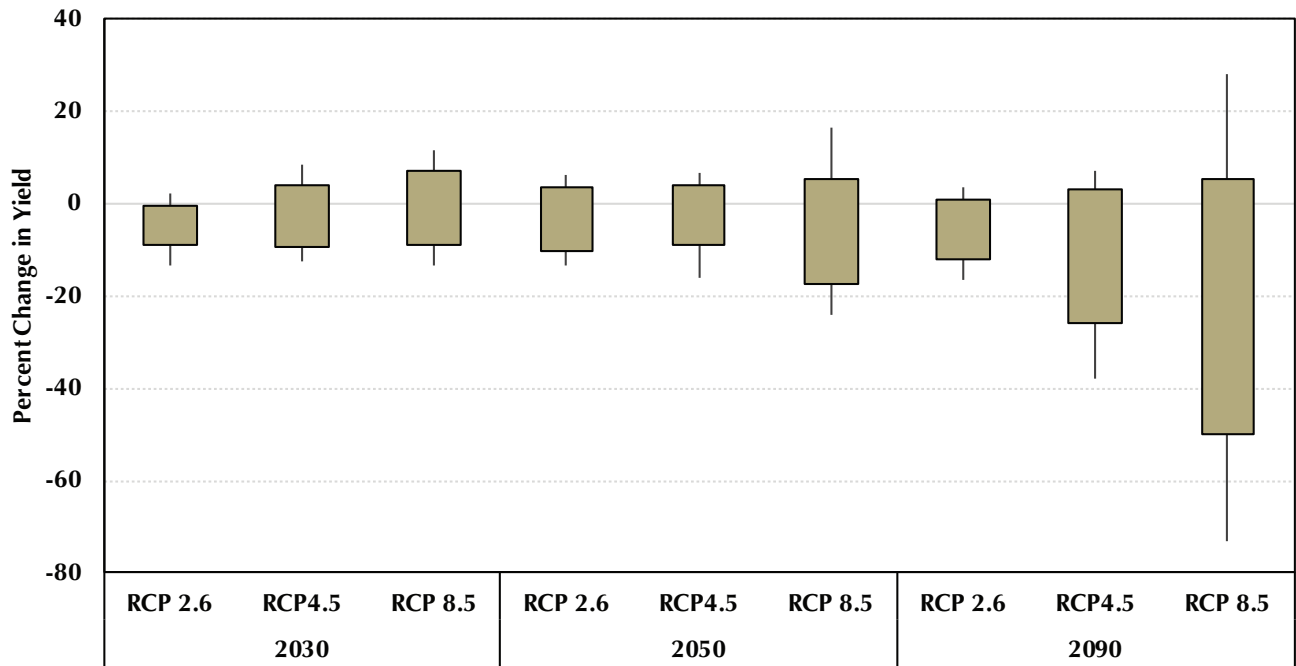
FIGURE 18: Changes in Crop Yields in Maryland in the 21st Century
