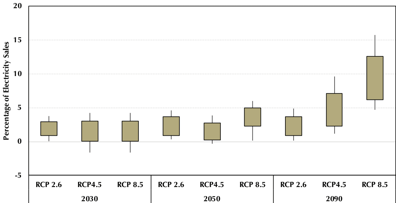
FIGURE 16 Changes in Electricity Sales in Maryland in the 21st Century
