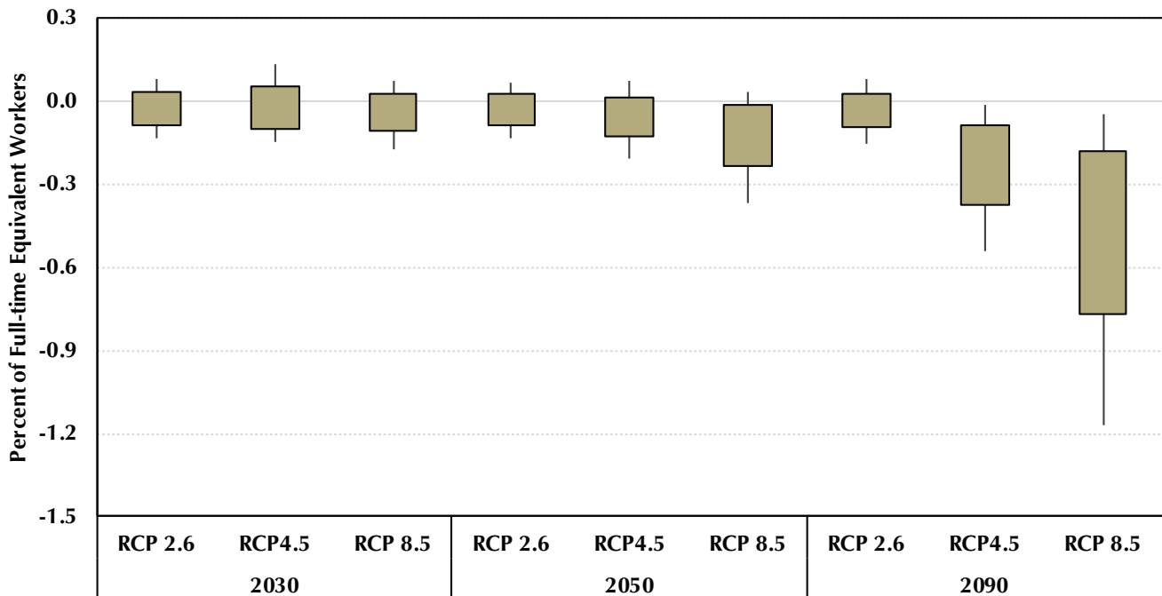
FIGURE 14: Changes in Labor Productivity in Maryland in the 21st Century
