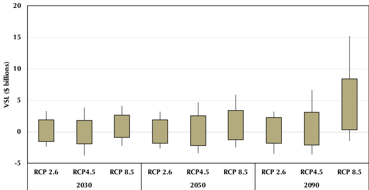
FIGURE 10: Costs Associated with Changes in Mortality in Maryland in the 21st Century
