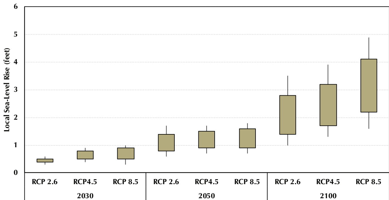
FIGURE 8: Projected Changes in Sea-Level Rise for Baltimore, MD in the 21st Century (Year 2000 Baseline)
