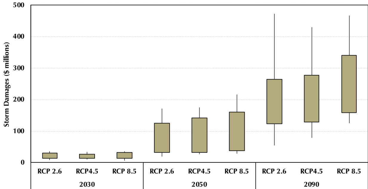
FIGURE 13: Increases in Costs associated with Storm Damage in Maryland for 2030, 2050, and 2100
