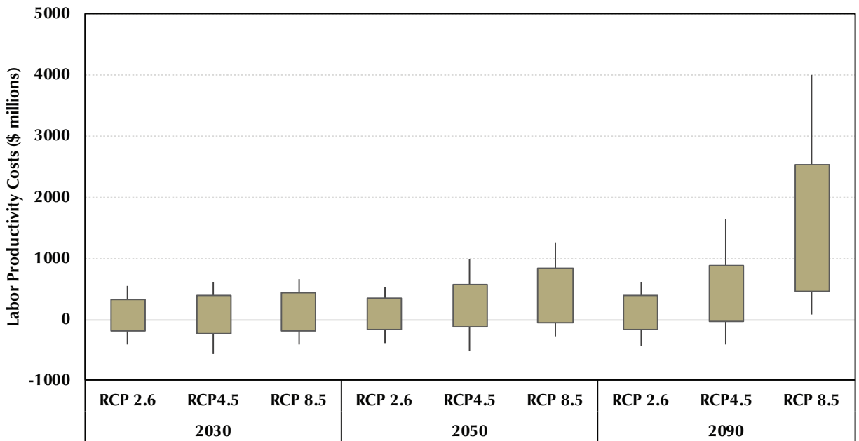
FIGURE 15: Costs Associated with Changes in Labor Productivity in Maryland in the 21st Century
